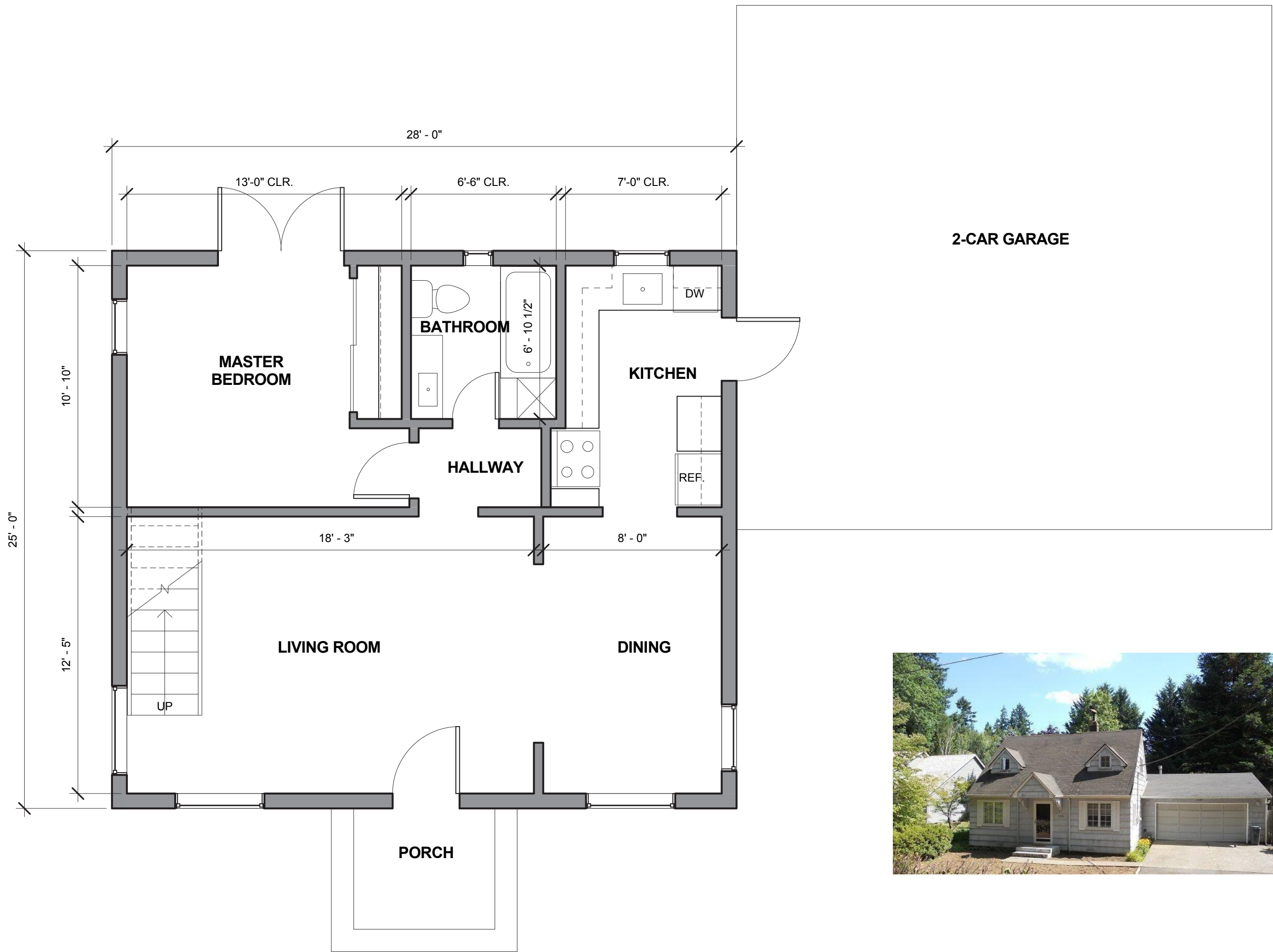
SUNSET DRIVE HOUSE- FIRST FLOOR
